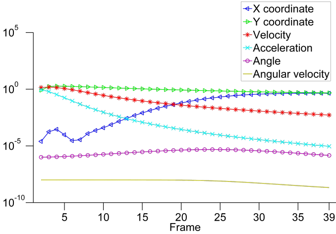
Fig. 11: Change of covariance matrix P_{k|k} components.
