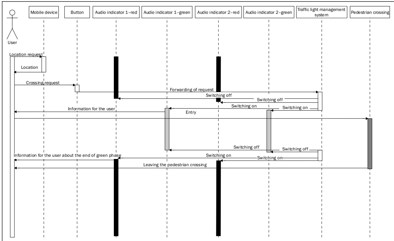
Figure 2 – Movement of users through traffic intersection (current method)
